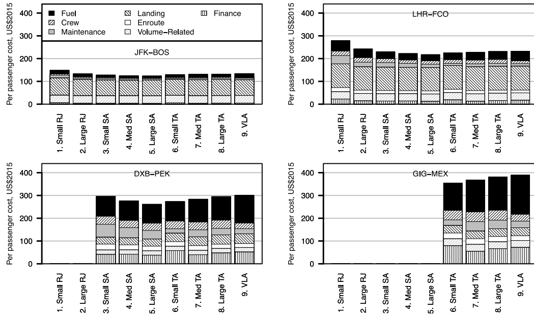
Figure 5. Direct and indirect operating cost model output for four example flight segments. Values are only shown where the stage length is below the maximum range of the reference aircraft 4 .
